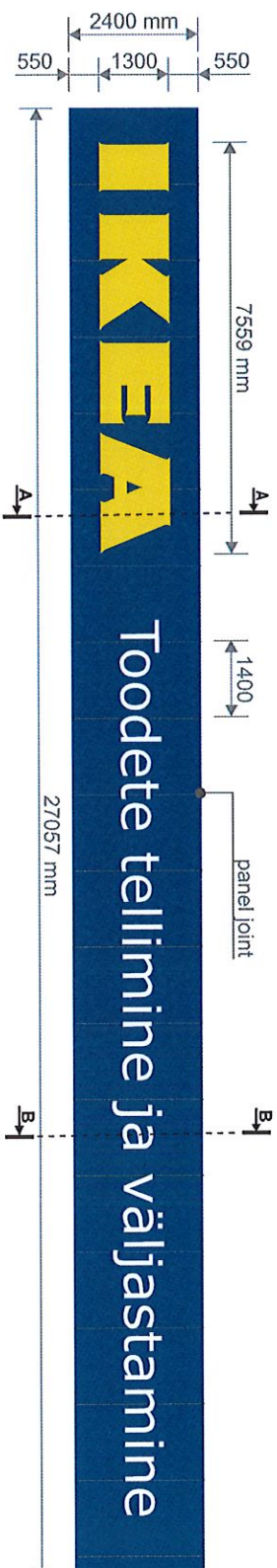
S1a internally illuminated channel letters panel size 27057 x 2400 mm, 2 pcs.
